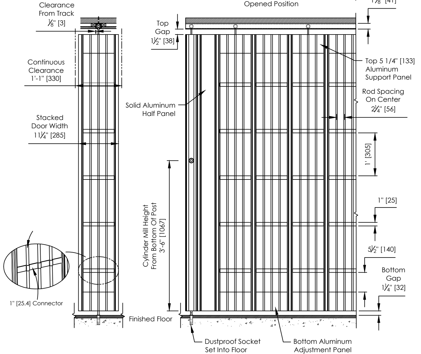
Opened Position
