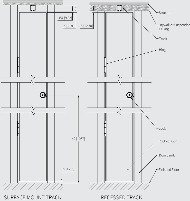
ELEVATION VIEW (RIGHT HAND DOOR)
