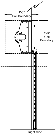
Right Side
