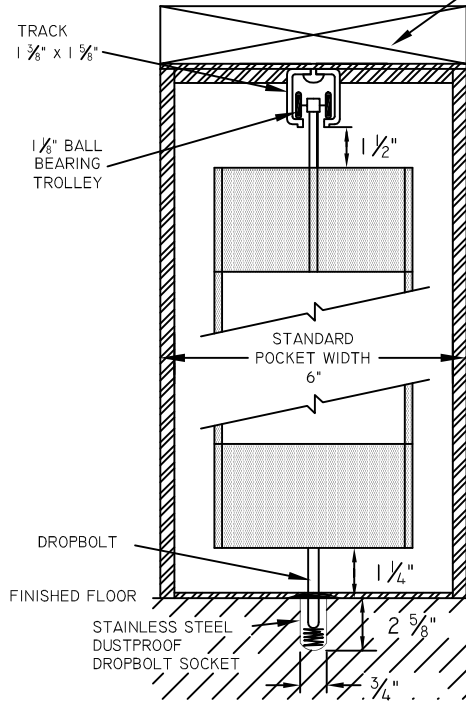
VERTICAL SECTION
